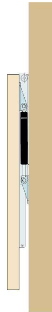
E14.5-GSK Side Elevation - Gas Strut Kit Standard Installation
